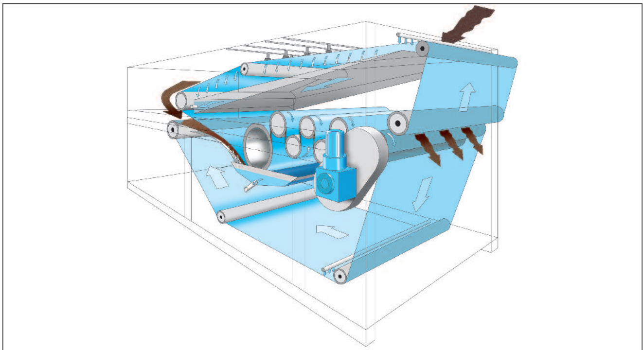
HUBER Bogenpress B-PRESS with 8 rolls
