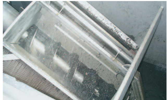
Floating and suspended material is retained in the screen basket. The tines mesh into the basket bars and ensure a complete automatic cleaning.
